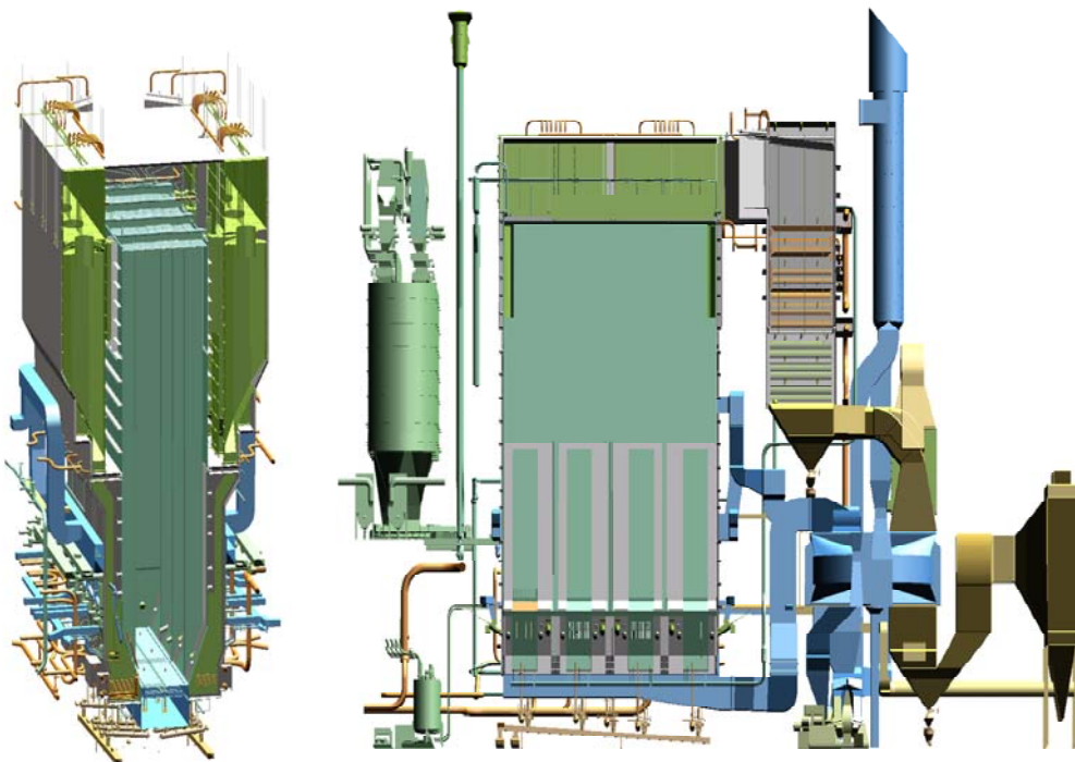
Figure 3 Łagisza CFB Boiler
